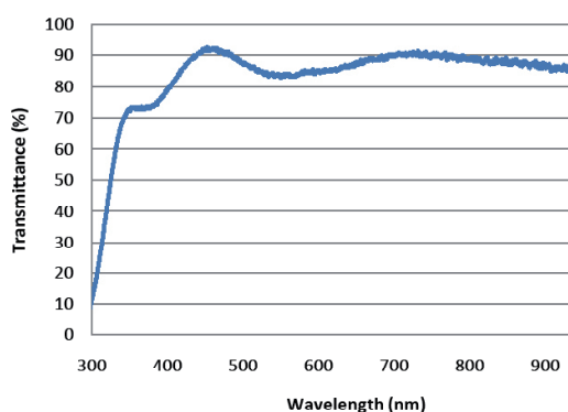
Transmission for ITO deposited at 200°C plus glass substrate Rs = 10 Ω/ (220nm)
